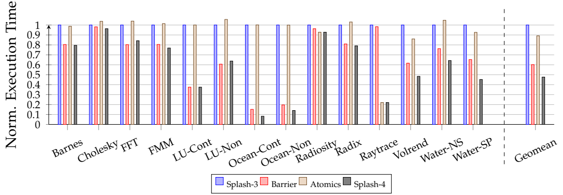
Figure 4.1: Execution time when upgrading Splash-3 barriers , atomics and both -Splash-4 (64-threads on AMD Epyc 7702P)
