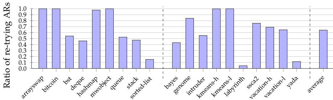
Figure 6.1: ARs that do not change their accessed cachelines on the first retry
