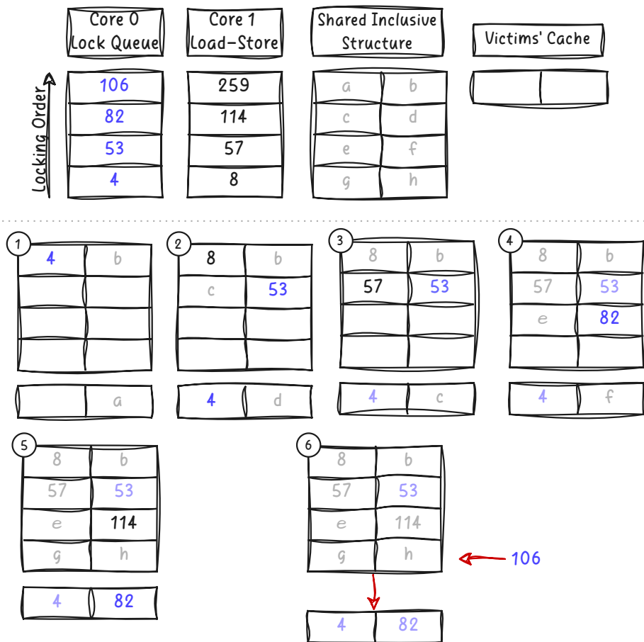
Figure 5.3: Deadlock scenario because the size limit of the MSHRs, caused by a core that is not locking addresses
