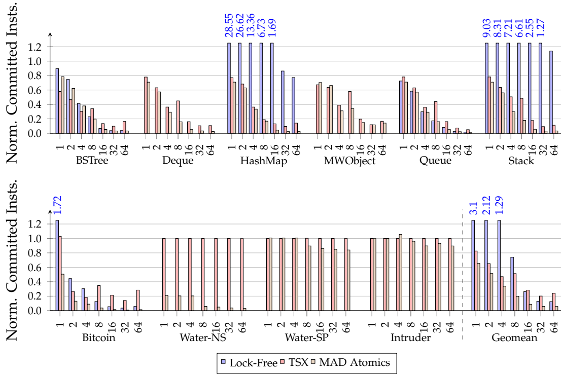
Figure 5.6: Normalized committed instructions (1 to 64 cores). Data is normalized against the lock version with the same core count. Deque, MWObject, Bitcoin, Water-NS, and Water-SP do not have a lock-free version. Intruder does not have a lock or lock-free version, it is normalized against TSX.
