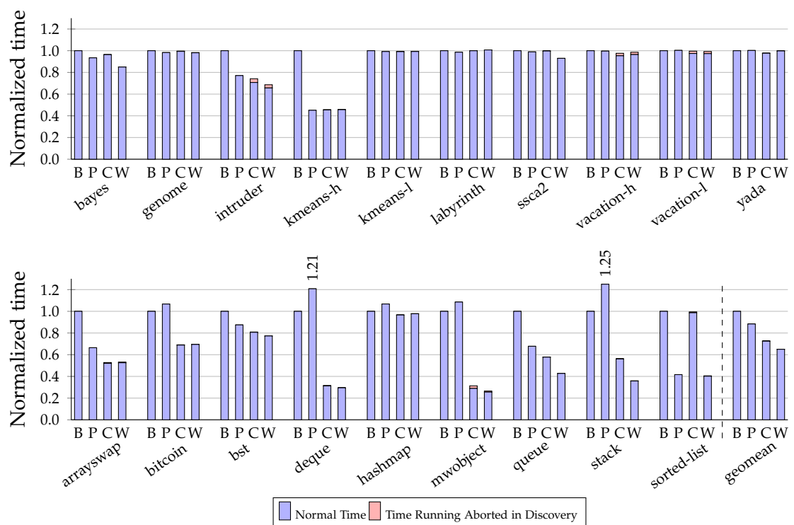
Figure 6.3: Normalized execution time
