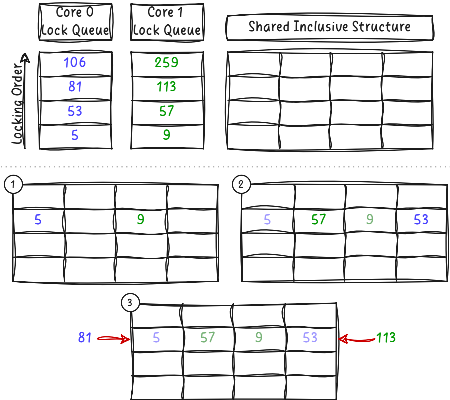
Figure 5.2: Shared structure conflict because multiple cores lock addresses in the same set of a shared inclusive structure.
