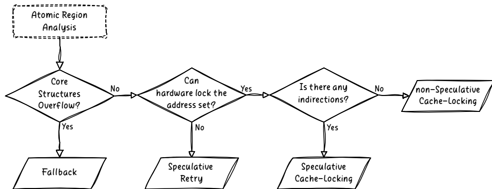
Figure 6.2: Decision tree of the execution modes of CLEAR
