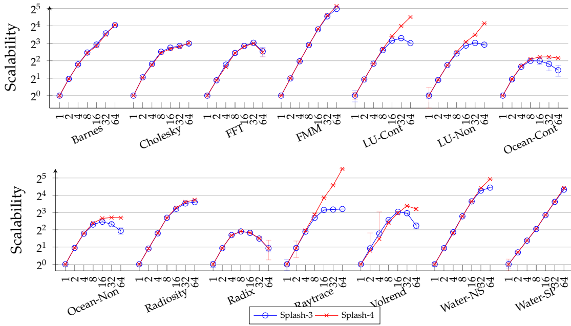
Figure 4.3: Splash-3 vs Splash-4 Scalability in simulated Intel Ice Lake (gem5-20)
