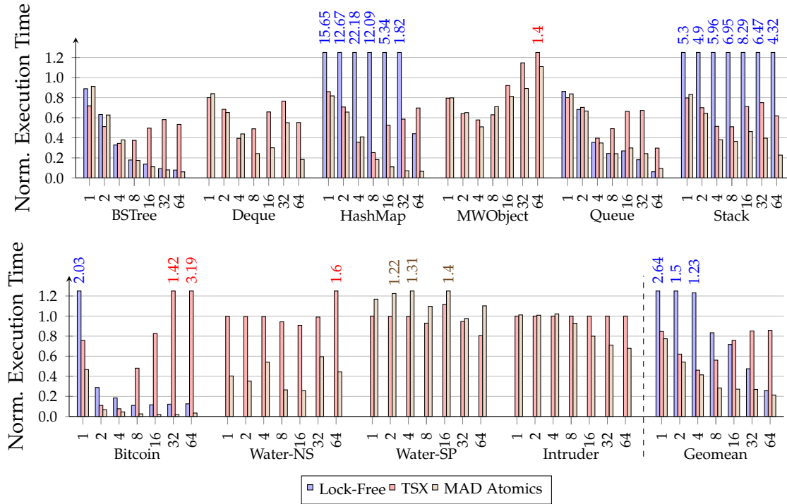
Figure 5.5: Execution time (1 to 64 cores). Data is normalized to the lock version with the same core count. Deque, MWOBJect, Bitcoin, Water-NS, and Water-SP do not have lock-free version. Intruder does not have a lock or lock-free version, it is normalized against TSX.
