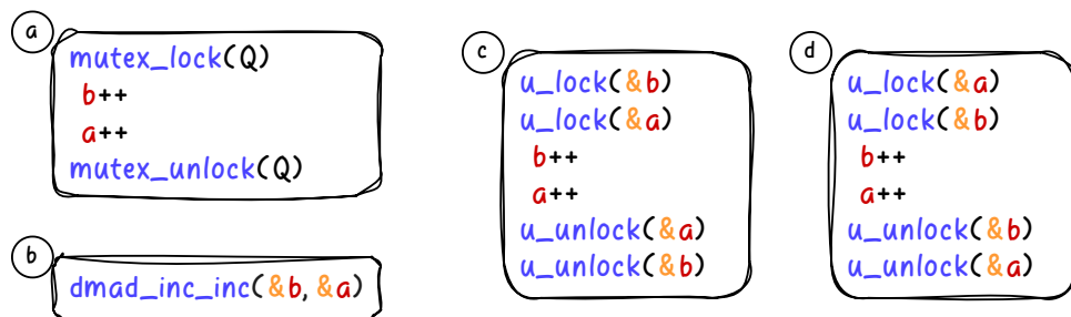
Figure 5.4: a) Critical section with mutex locks; b) MAD atomic instruction; c) micro-ops generated by the MAD atomic; d) run-time order of instructions.
