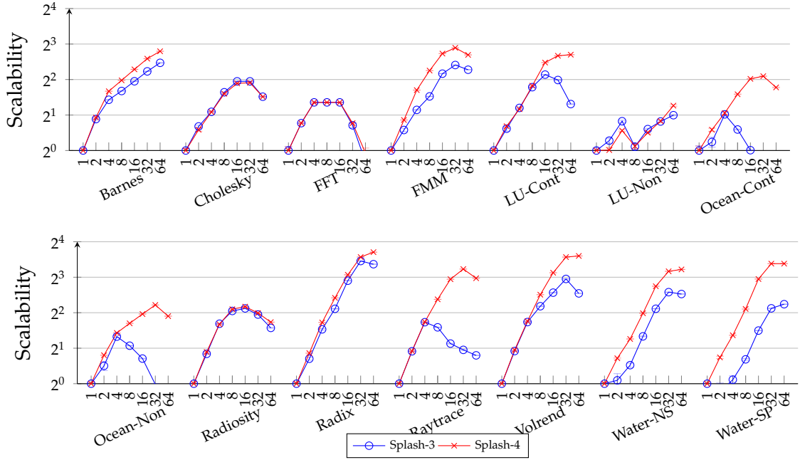
Figure 4.2: Splash-3 vs Splash-4 Scalability on AMD Epyc 7702P
