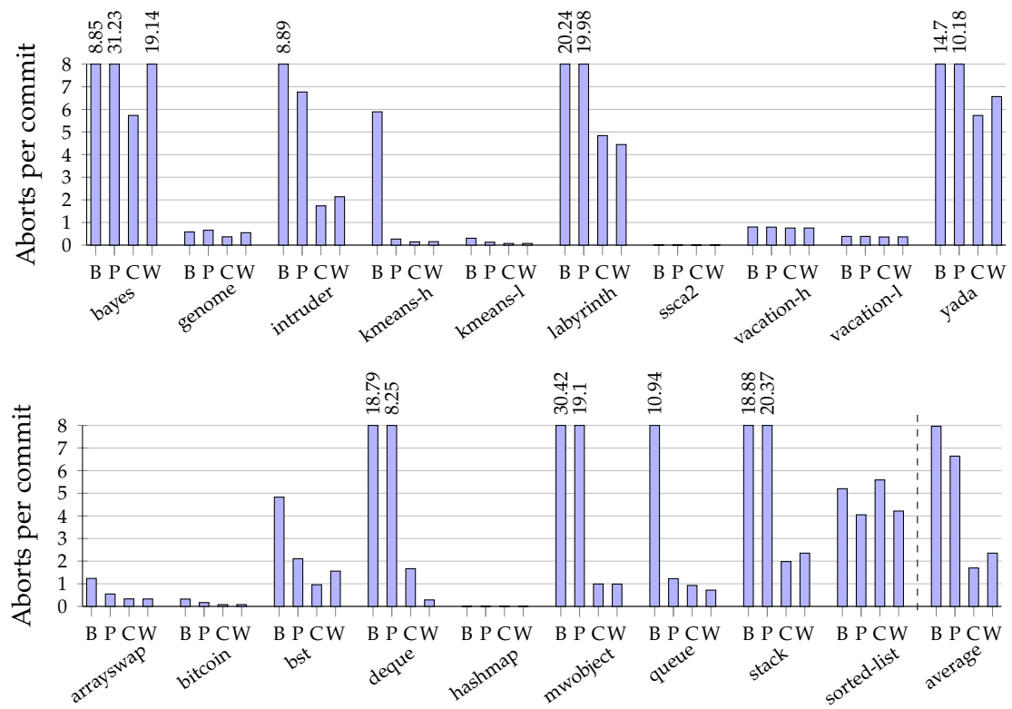
Figure 6.4: Aborts per Committed Transaction
