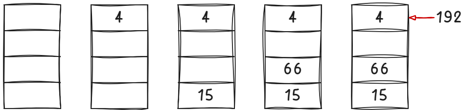
Figure 5.1: Directly mapped structure causing a conflict that prevents locking all addresses despite having enough space.
